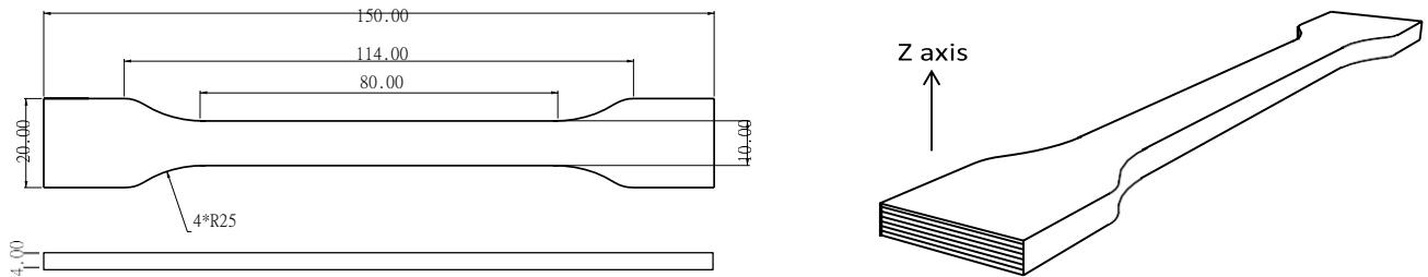
Fig 1. Tensile testing specimen
